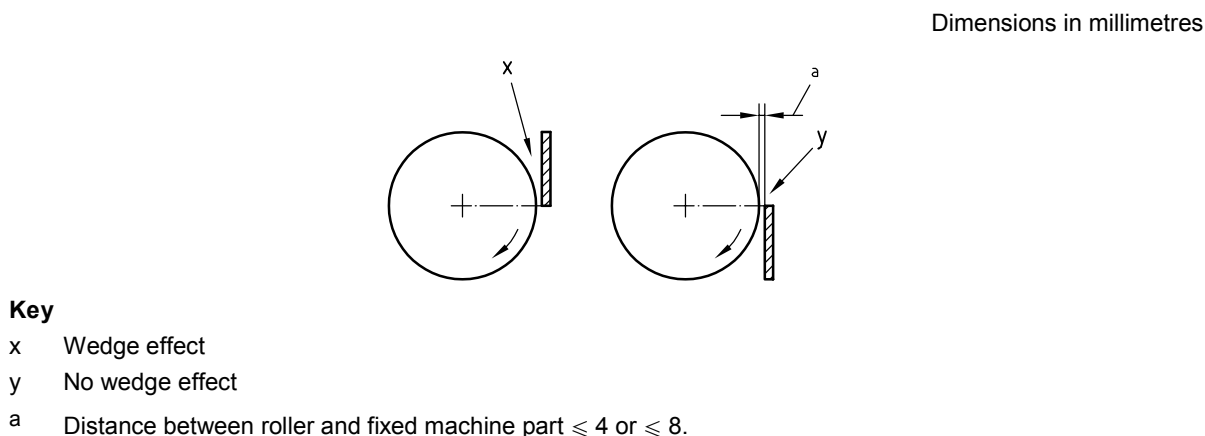
Figure 7 — Avoidance of wedge effect
